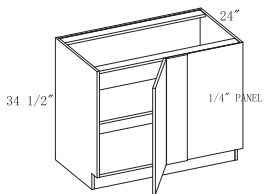
Base Blind Cabinet
