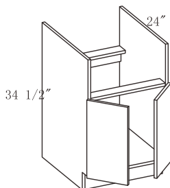
Farm Sink Base Cabinet 2 doors
